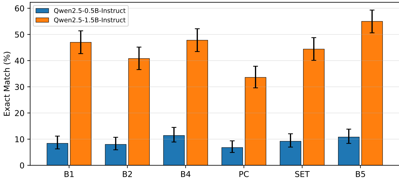
Per-chunk (PC) vs set-level (SET) verification, 95% Wilson intervals
