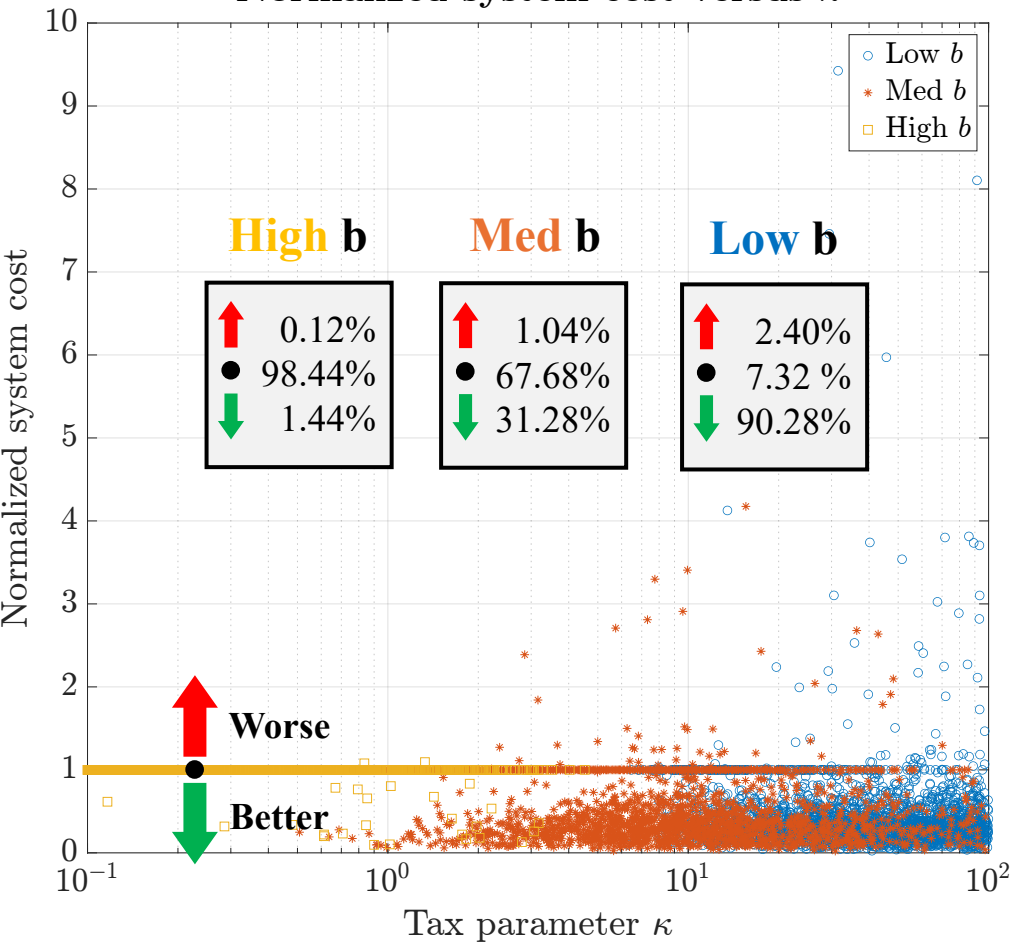
Normalized system cost versus \kappa
