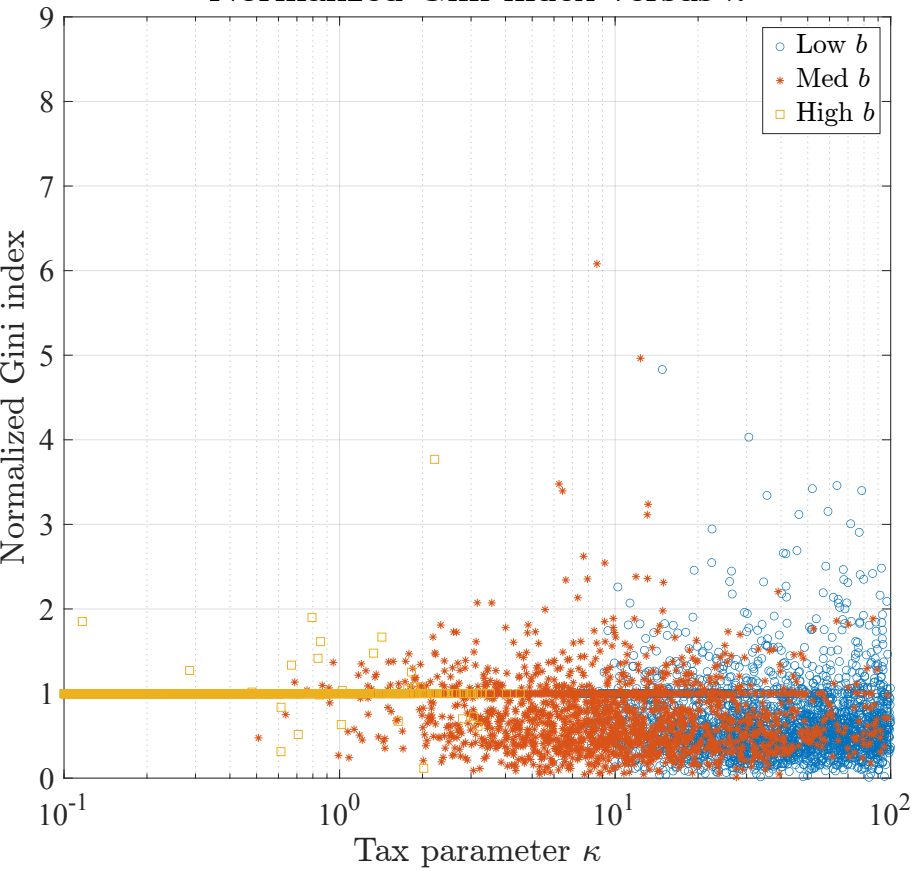
Normalized Gini index versus \kappa
