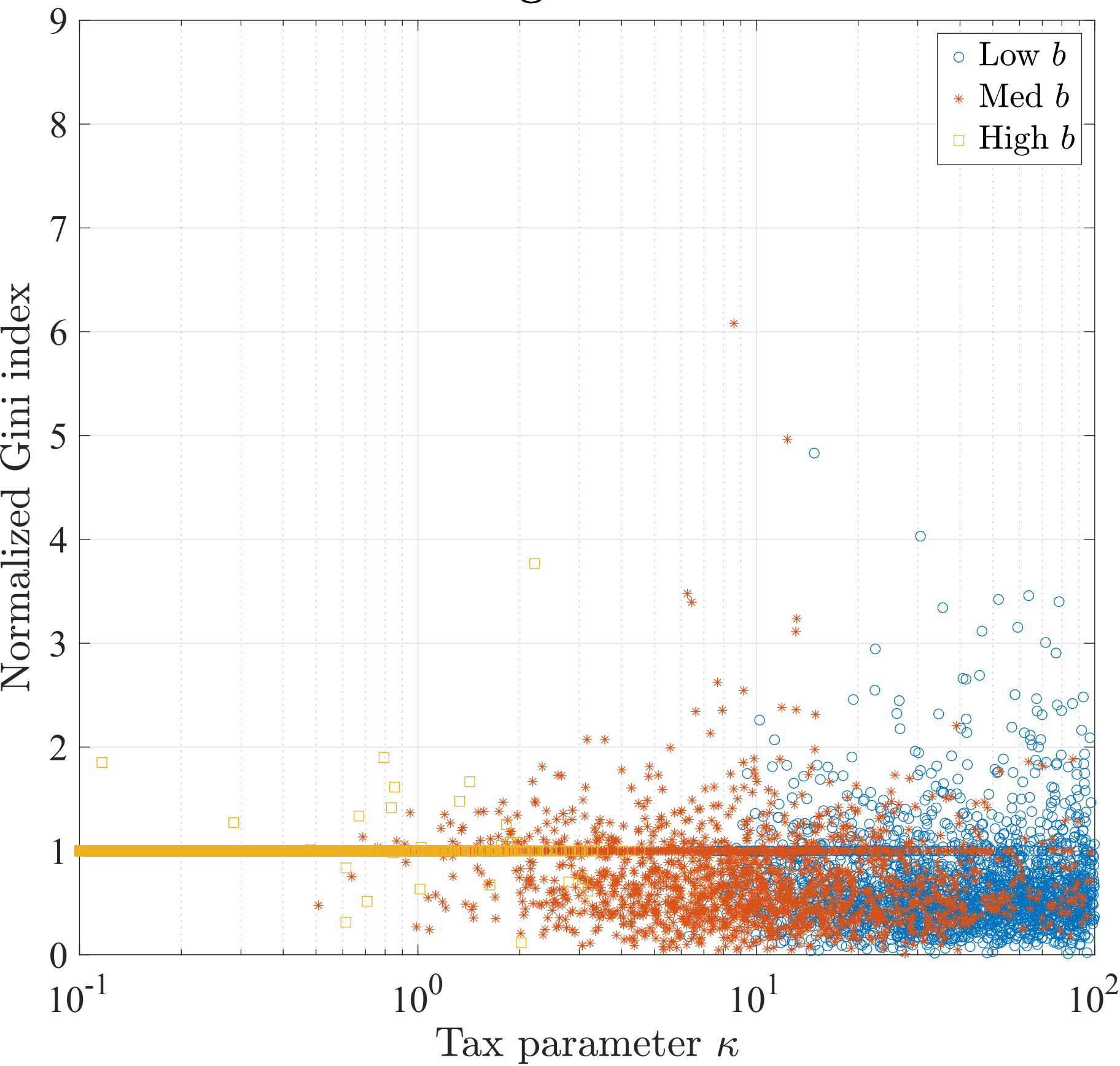
Normalized gini index versus \kappa
