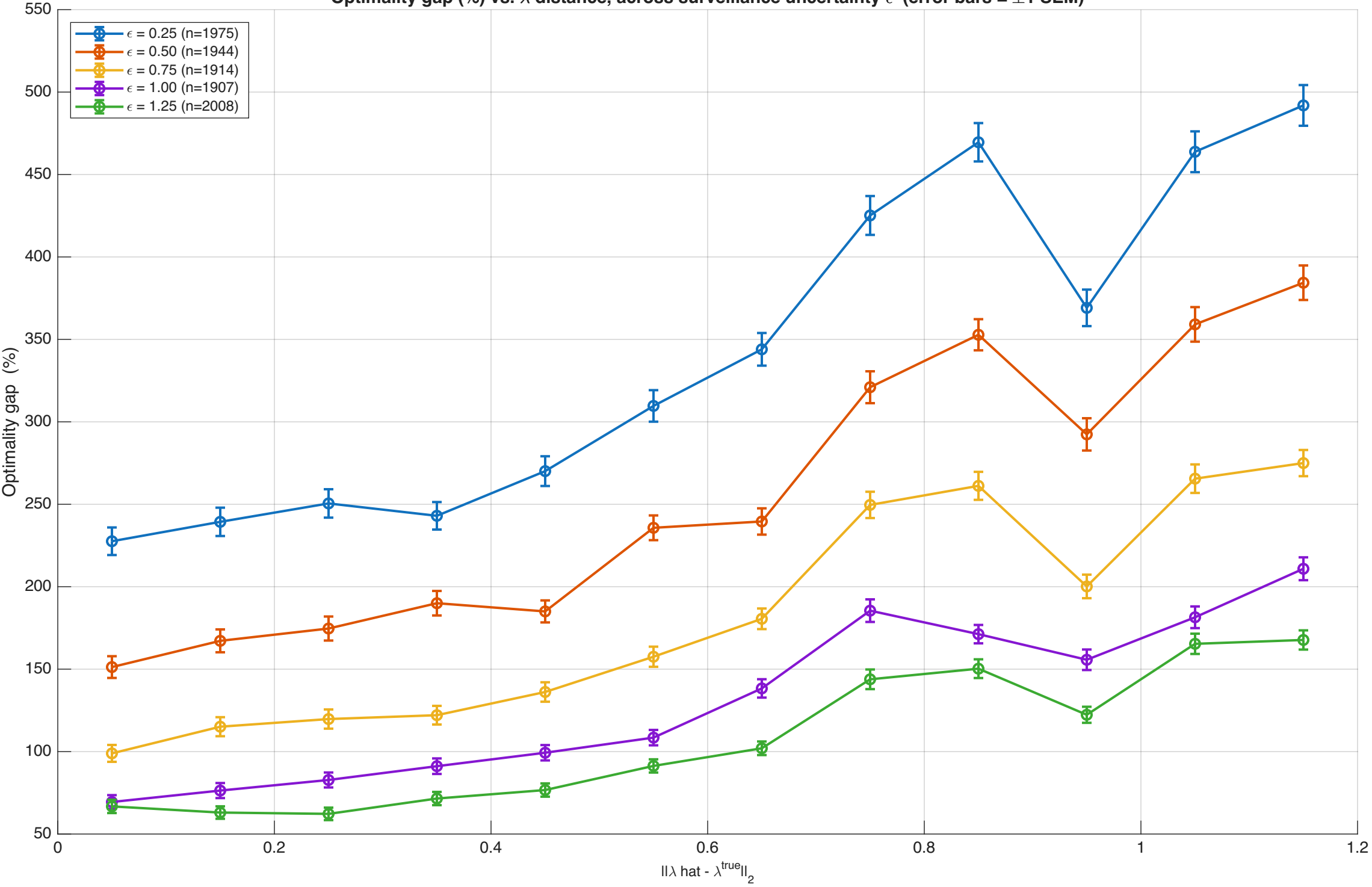
Optimality gap (%) vs. \lambda distance, across surveillance uncertainty \epsilon (error bars = \pm 1 SEM)
