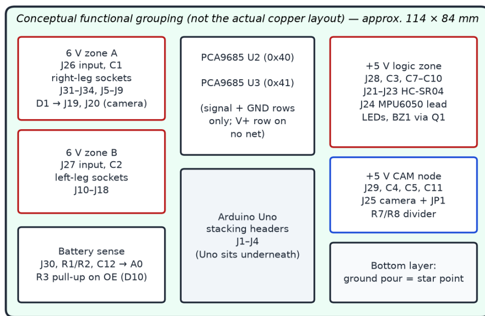
Figure 6.2: Functional grouping of the shield (conceptual — the actual placement is shown in the KiCad layout figures)
