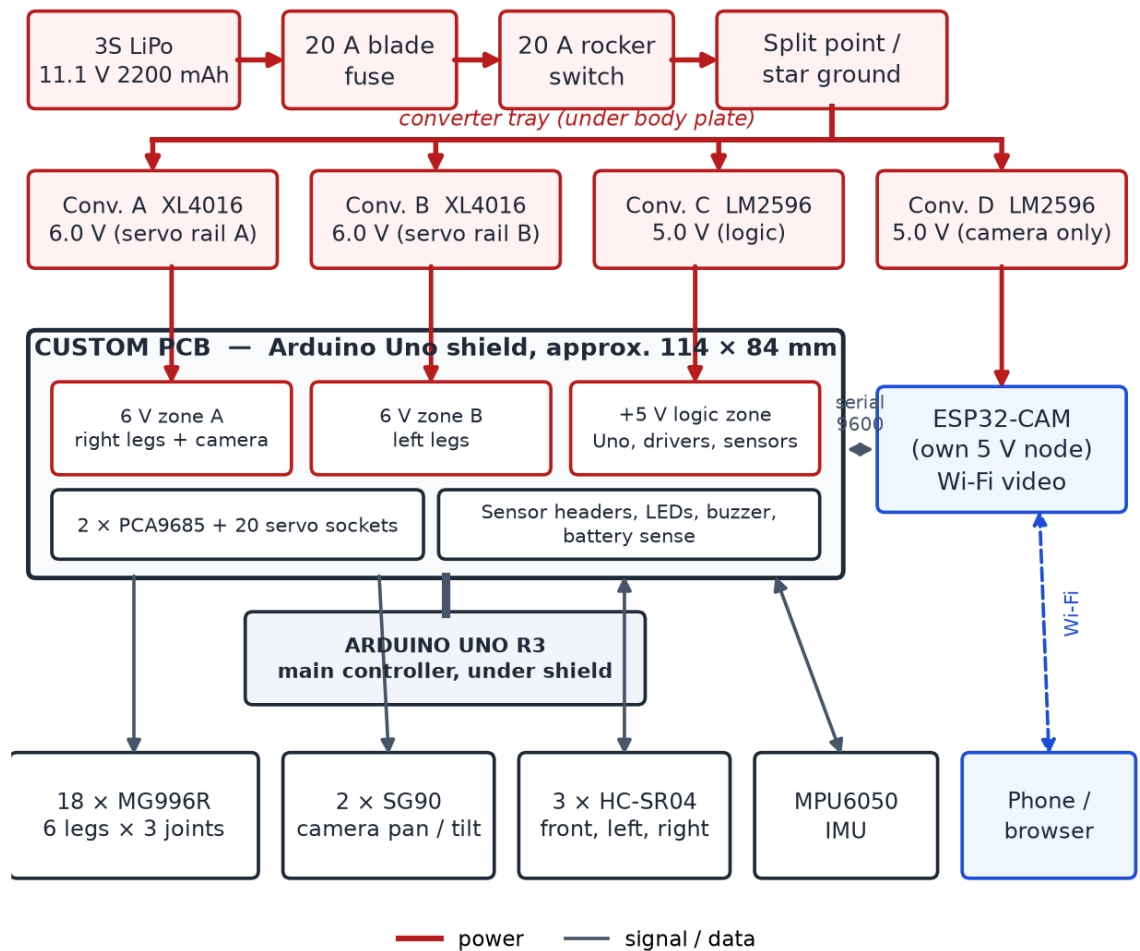
Figure 4.1: Overall system block diagram of the planned hexapod (based on the architecture in our build plan)
