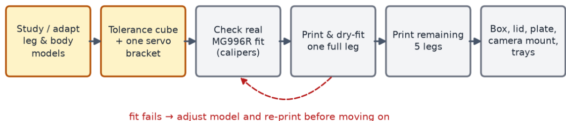
Figure 8.2: Planned 3D printing workflow — each step is checked before the next
