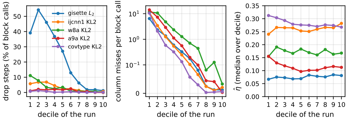
Figure 4: Along the run at k = 16 (deciles of the iteration count, one line per cell): fraction of block calls that are drops, column misses per block call, and the effective correlation \hat{\eta} . Drops and misses are paid while the support is built and become rare once it has settled, the shape Theorem 15 describes, most clearly on gisette, ijcnn1 and w8a; \hat{\eta} is nearly constant along the run (a9a falls from 0.16 to 0.10 over the first five deciles, covtype from 0.31 to 0.27).
