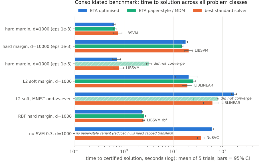
Figure 3: Time to certified solution on seven problem classes: the optimised configuration vs the toward-step or single-MDM configuration vs the best standard solver per class (settings in Section 8.3); five trials per class, mean with 95% CI. The \nu -SVM row has no toward-step bar because the algorithm of Gupta and Kalantari (2026) has no reduced-hull variant (reduced hulls need capped transfers).
