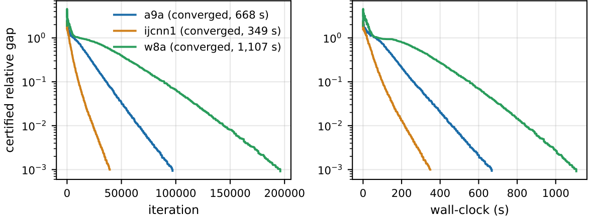
Figure 1: Certified relative gap of ETA on a9a, w8a and ijcnn1 ( L_2 , C = 0.1 , uncapped, seed 0), versus iteration and wall-clock: linear-rate convergence in the dense-support regime, reaching the certified 10^{-3} in 349–1,107s against the 600s cap of Table 7.
