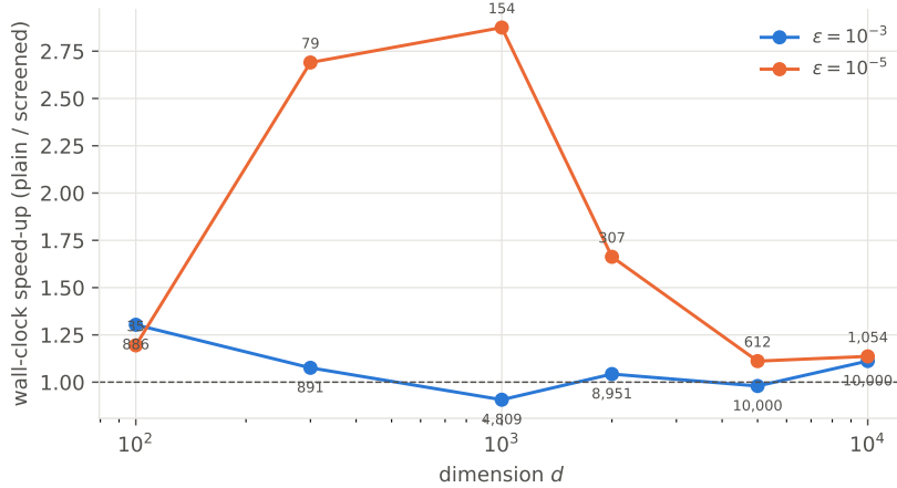
Figure 2: Safe screening on the separated synthetic protocol ( n=10,000 , two trials): wall-clock speed-up of screening versus dimension at \varepsilon = 10^{-3} and 10^{-5} ; labels are surviving points of 10,000. Made with the toward-step solver of the development phase ( src/shrink_benchmark.py ); the rule and its activation do not depend on the step, and Table 3 gives the released solver on real data.
