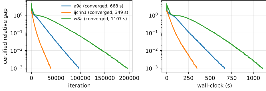
Figure 1: Certified relative gap of ETA on a9a, w8a and ijcn1 ( L_2 , C = 0.1 , uncapped, seed 0), versus iteration and wall-clock: linear-rate convergence in the dense-support regime, reaching the certified 10^{-3} in 349–1,107s against the 600s cap of Table 5.
