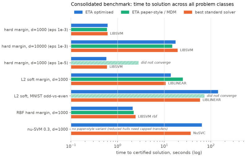
Figure 3: Time to certified solution on seven problem classes: optimised ETA vs the paper-style configuration vs the best standard solver per class. The \nu -SVM row has no paper-style bar because the toward-step algorithm of [2] has no reduced-hull variant (reduced hulls need capped transfers).
