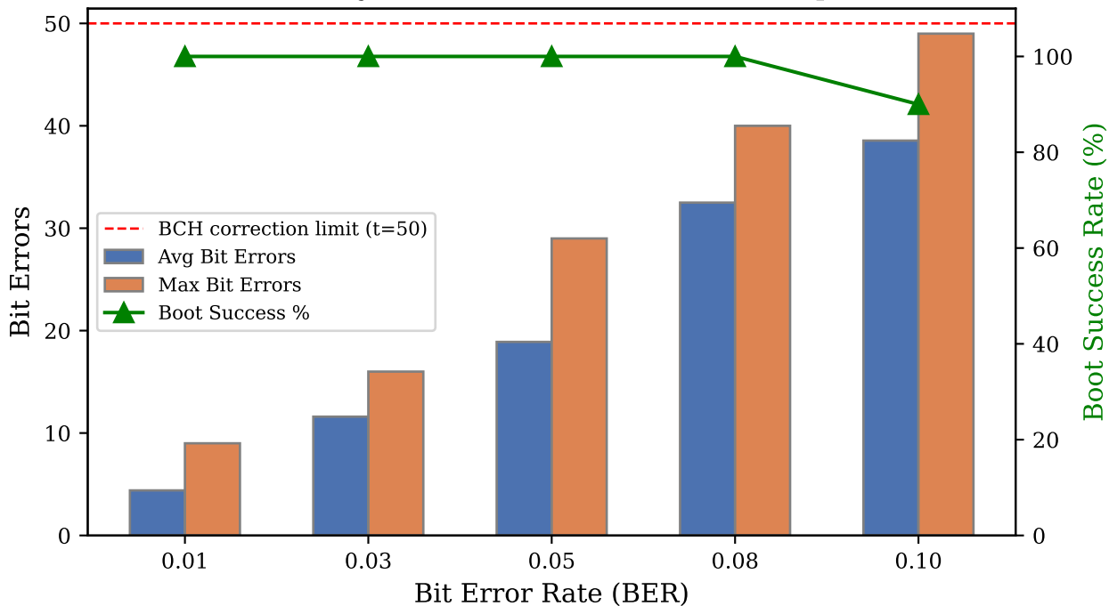
PUF Reliability vs Bit Error Rate (10 Devices per BER)
