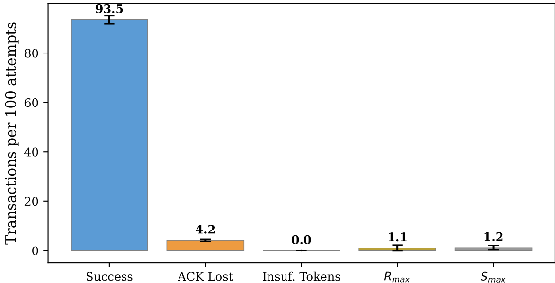
Transaction Outcome Distribution (mean \pm \sigma , 10 seeds \times 100 txns)
