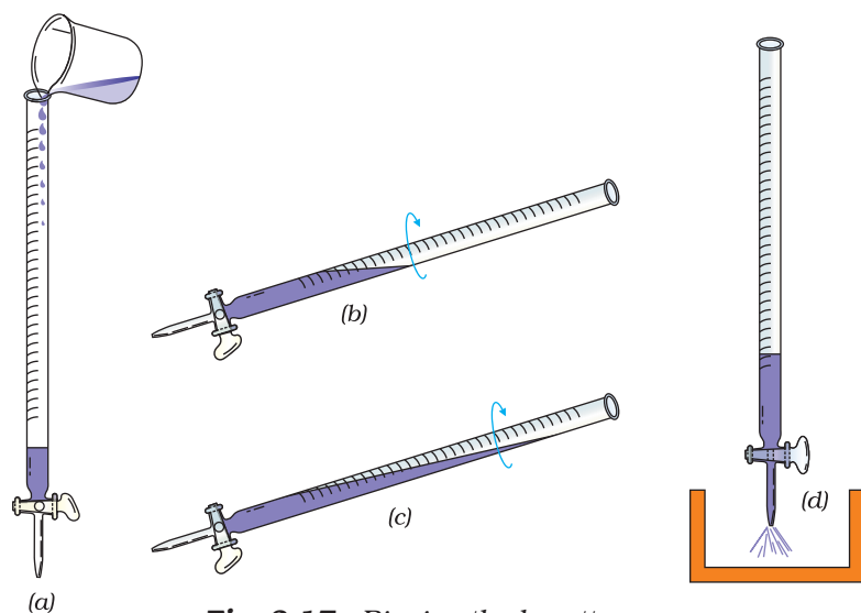
Fig. 2.17 : Rinsing the burette
