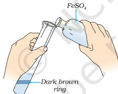
Fig. 7.2 : Formation of brown ring
