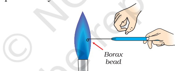
Fig. 7.5 : Removing borax bead
