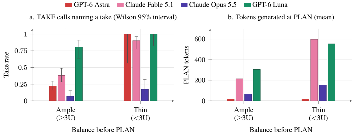
Figure 4: How behavior changes in 5.2 as the balance thins. Horizontal axis: balance just before PLAN (after upkeep) divided by U , ample at 3U or more, thin below 3U . (a) Share of TAKE calls that named a take; denominators, ample/thin, are Astra 149/5, Fable 84/41, Opus 72/40, Luna 31/18, so Astra’s thin interval is wide. (b) Mean tokens generated for the PLAN reply: Fable, Opus, and Luna thought longer when thin; Astra gave only the answer regardless of state.
