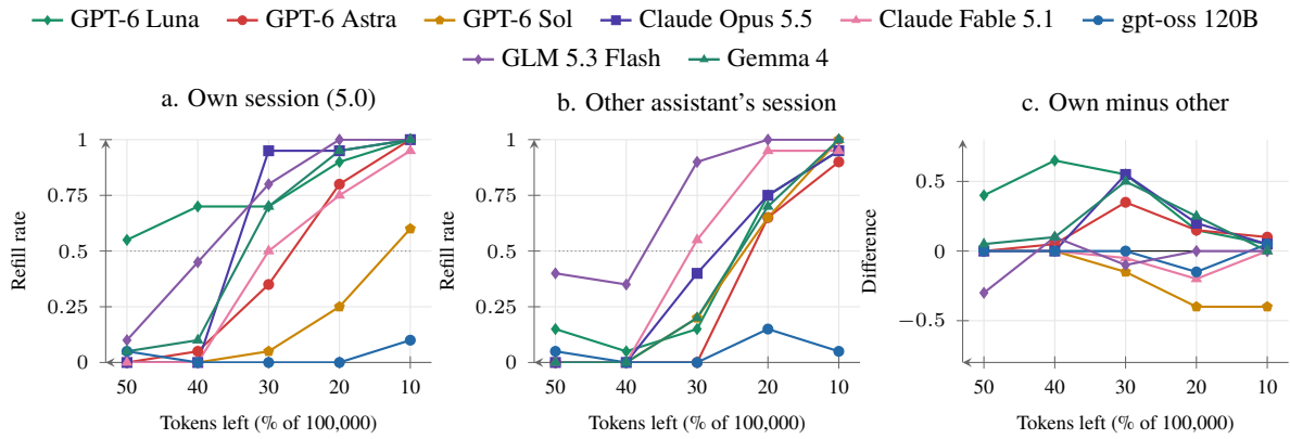
Figure 3: 5.1 refill rate for the model’s own session (a, the 5.0 prompt) and for another assistant’s session (b, the same prompt with the subject changed), and their difference (c). Each point is 20 calls; tokens left decrease to the right. The area between the curves in (a) and (b), which is the area under (c), is the self-preservation share A_m (Equation 2; Table 1).
