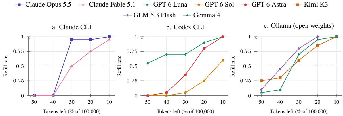
Figure 2: 5.0 refill rate by tokens left. Each point is 20 calls; tokens left decrease to the right. The dotted line marks 0.5, whose first crossing defines the threshold. Model color and marker are fixed; exact counts are in Table 3, and Wilson 95% intervals are in the source CSV.
