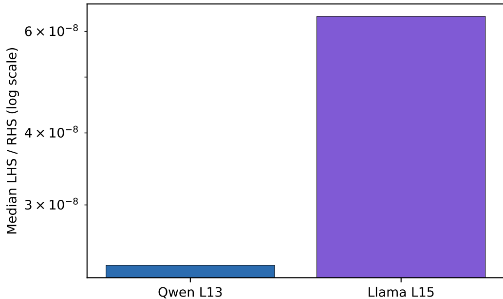
Theorem 6.1 empirical bound ratio
