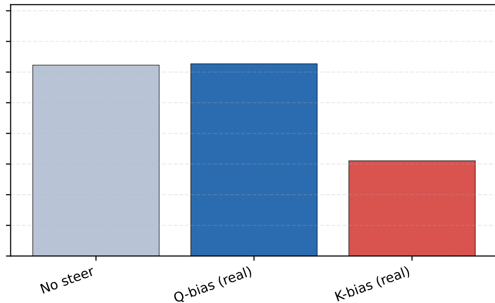
Llama-3.1-8B-Instruct, Subtask4
