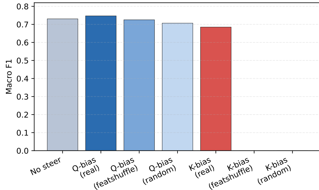
Qwen2.5-7B-Instruct, Subtask4
