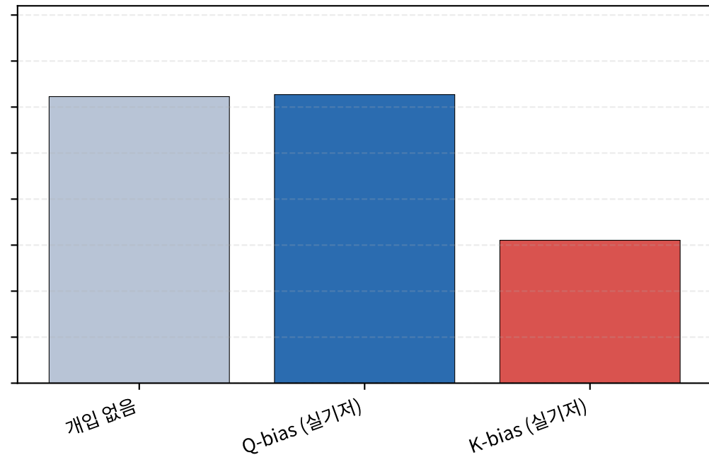
Llama-3.1-8B-Instruct, Subtask4
