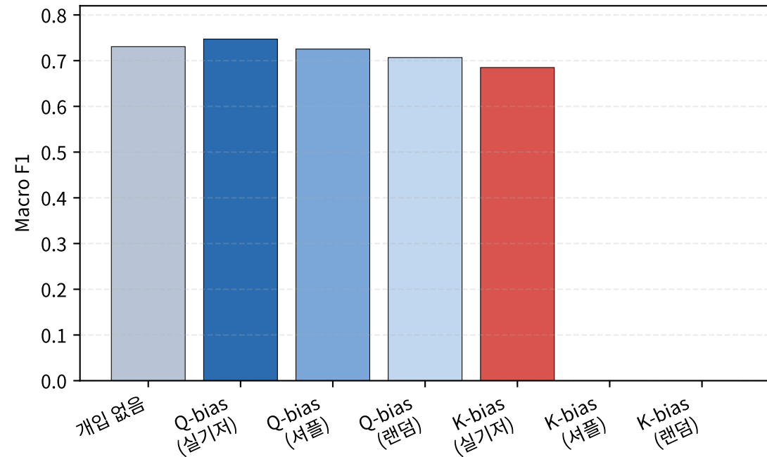
Qwen2.5-7B-Instruct, Subtask4
