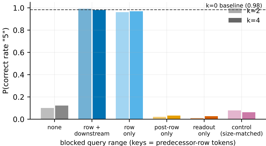
Attention-mask knockout: recovery by blocked query range
