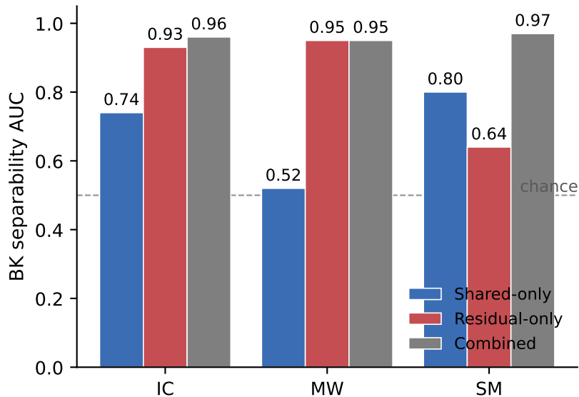
Shared / Residual decomposition (Gemma L22)
