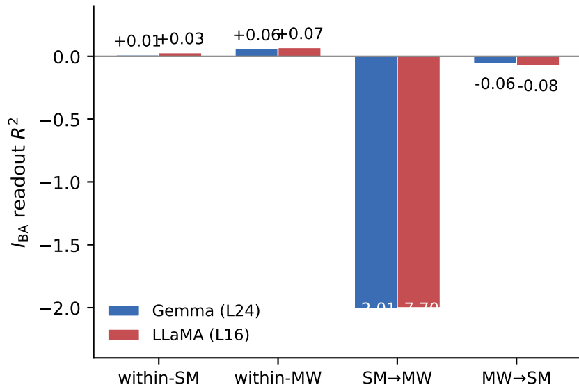
Cross-task readout transfer
