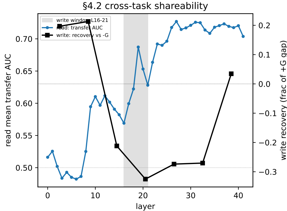
gemma: $4 read (all layers) vs causal write recovery (window center)
