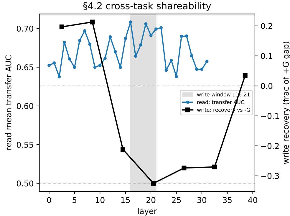
llama: §4 read (all layers) vs causal write recovery (window center)
