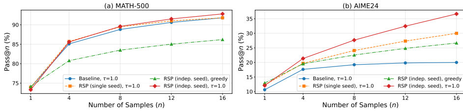
Figure 3: Pass@ N scaling on (a) MATH-500 and (b) AIME24 with Qwen2.5-Math-1.5B-Instruct, N = 16 samples per problem. Baseline: temperature sampling only. Fixed seed: single RSP shared across samples combined with temperature. Indep. seed: a different RSP per sample, with or without temperature.
