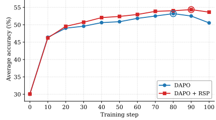
Figure 4: Five-benchmark average accuracy on Qwen2.5-Math-7B. DAPO + RSP reaches a higher peak (step 90) and stays stable through step 100.
