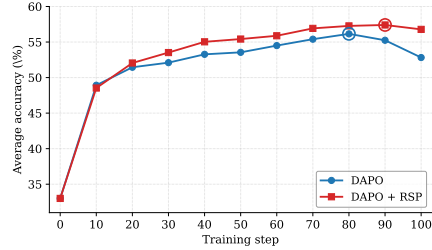
Figure 5: Seven-benchmark average accuracy on Qwen2.5-Math-7B. DAPO + RSP reaches a higher peak (step 90) and stays stable through step 100, while DAPO declines after step 80.
