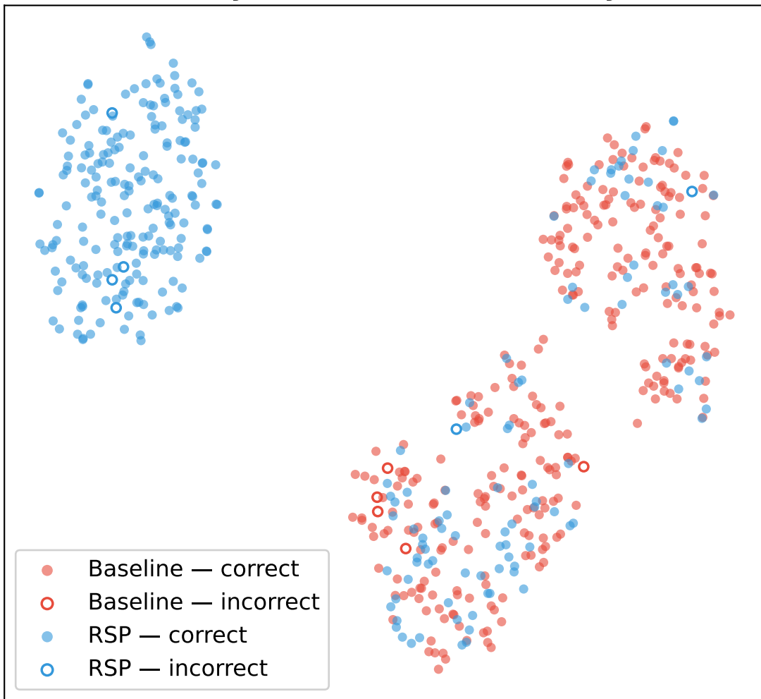
(a) t-SNE Projection of Solution Trajectories
