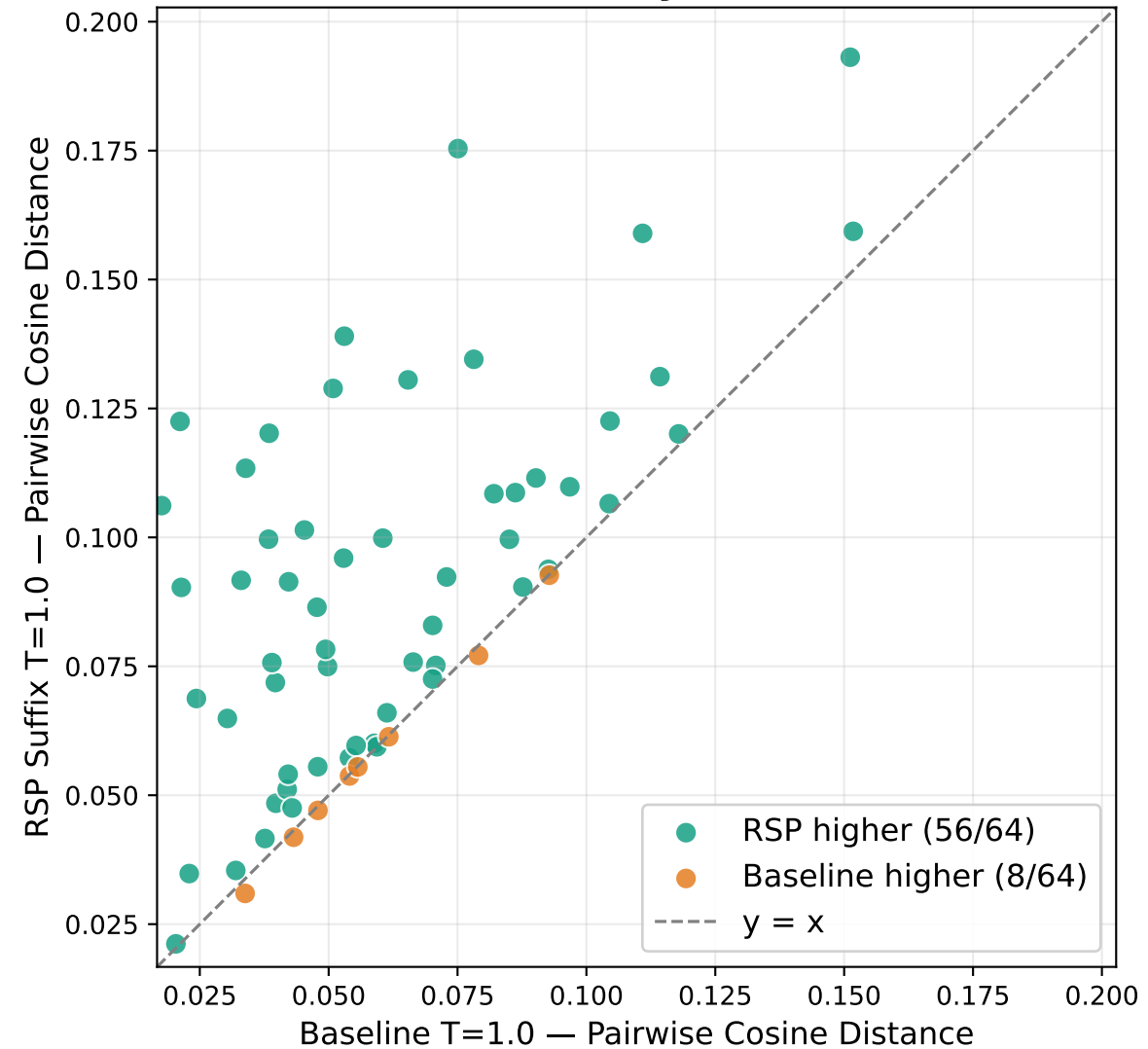
(c) Pairwise Diversity Across Problems
