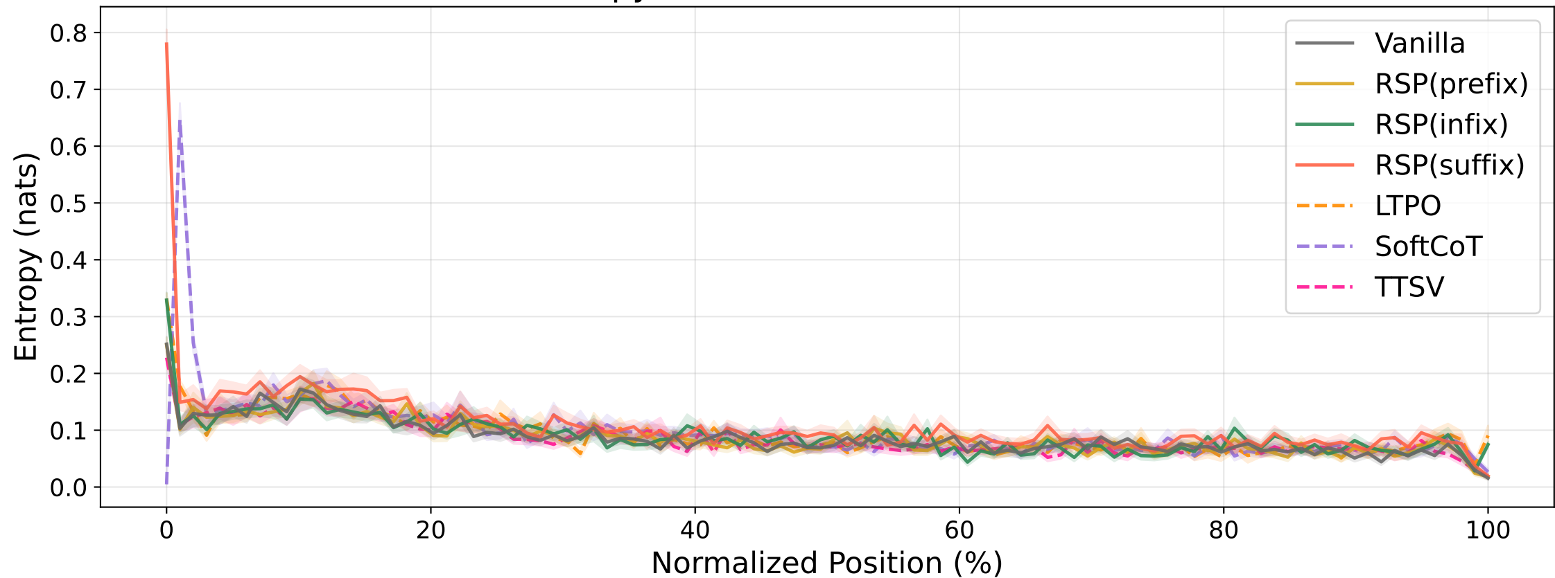
Per-token Entropy over Generation (Normalized Position)
