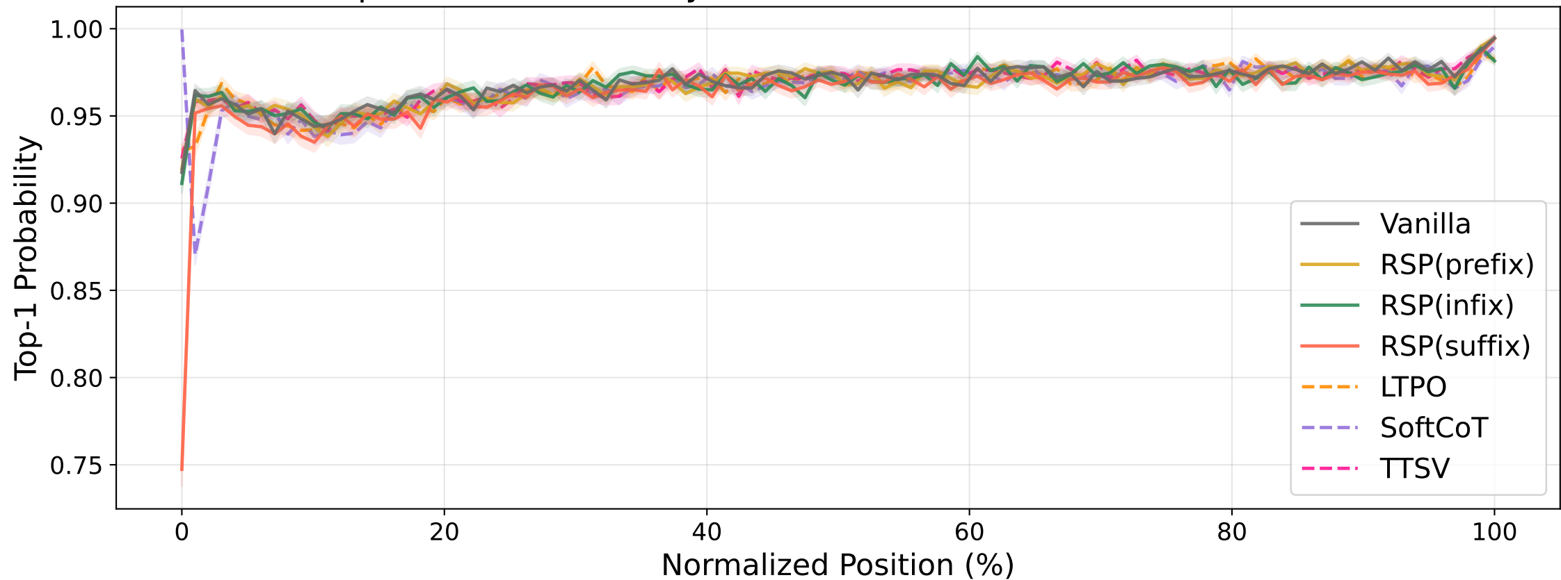
Top-1 Token Probability over Generation (Normalized Position)
