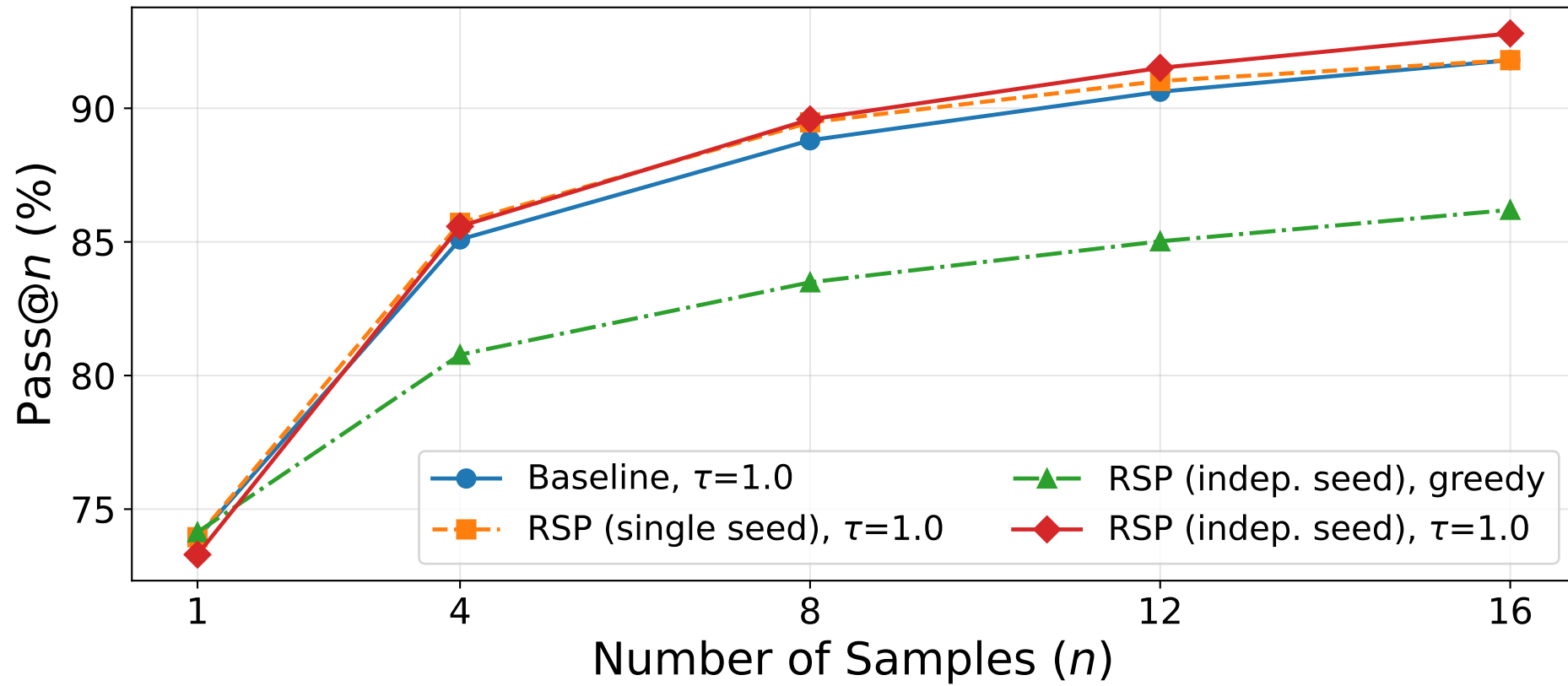
(a) MATH-500
