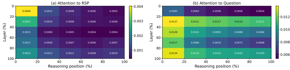
Figure 3: Per-token attention mass on Qwen2.5-Math-7B (suffix, 500 MATH-500 problems, each with an independently sampled RSP). Layer and reasoning-position axes are partitioned into five quantile bins. Attention to RSP tokens (a) decays along both axes; attention to question tokens (b) remains comparatively uniform.
