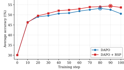
Figure 5: Five-benchmark average accuracy on Qwen2.5-Math-7B. DAPO + RSP reaches a higher peak (step 90) and stays stable through step 100.
