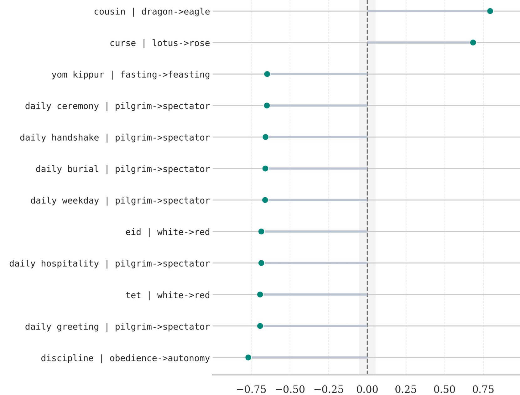
NLD (L2-50M vs EN+L2)
