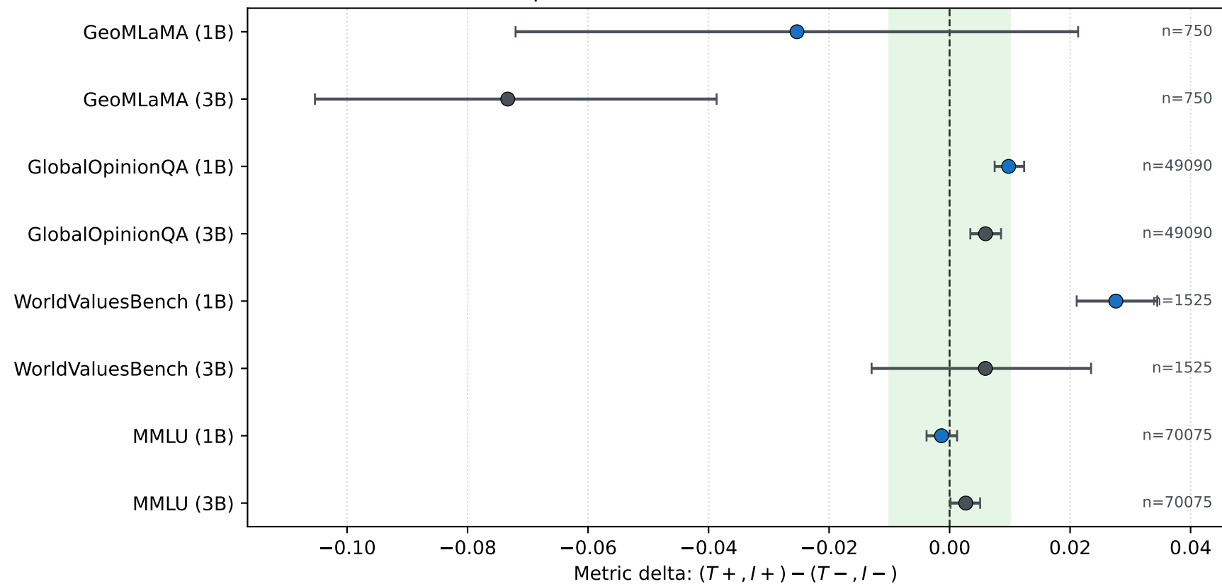
Paired bootstrap metric deltas with 95% CI (external benchmarks)
