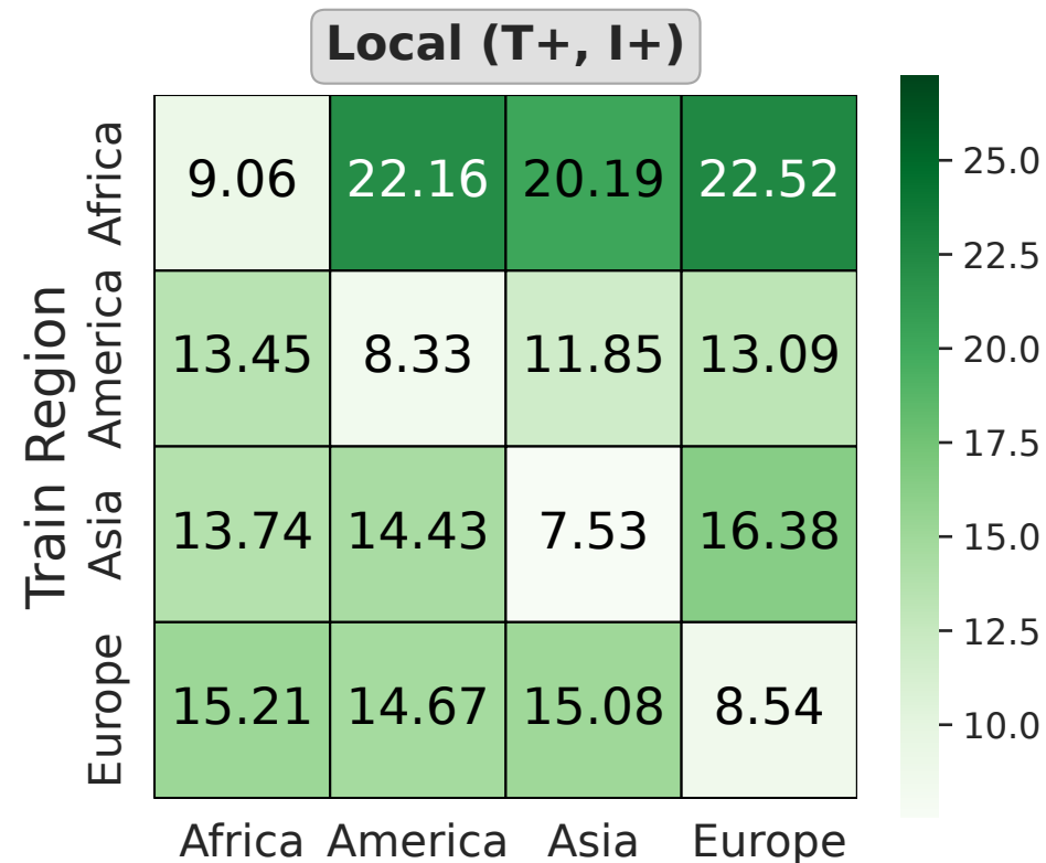
Training with metadata
