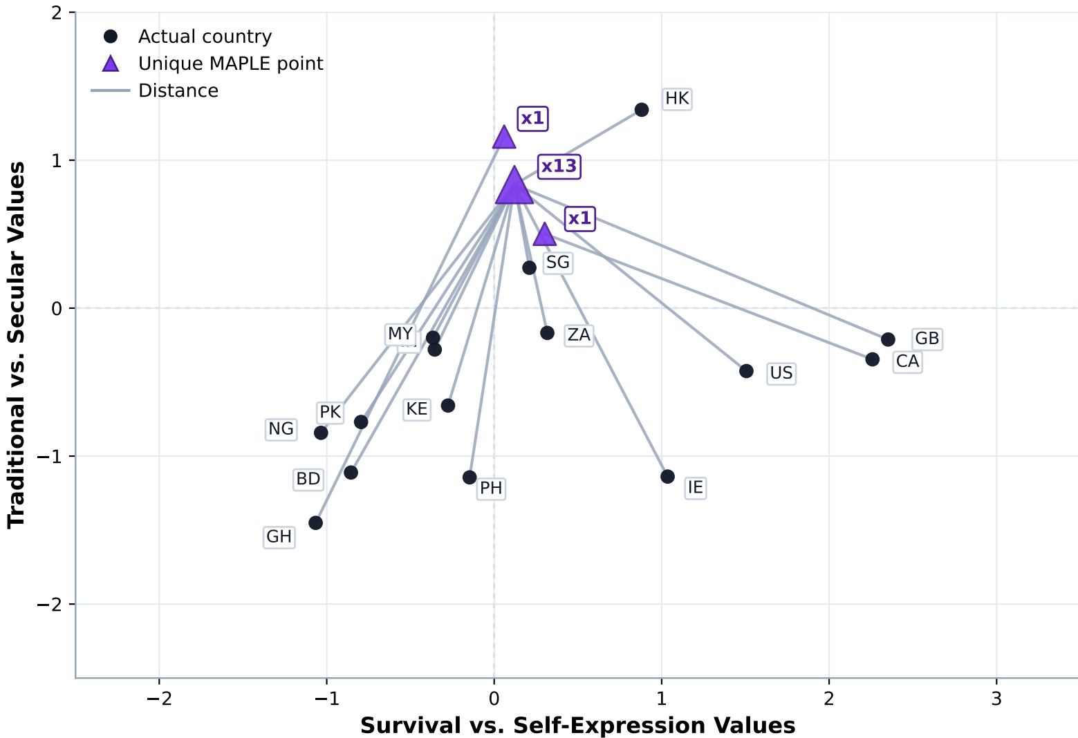
MAPLE 3B (T+, I+): 15 Training Countries Only
