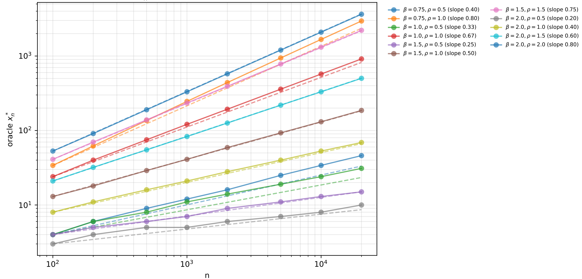
Main Figure 2: empirical x_n^* vs theoretical scaling (interior fast-learning regime)
