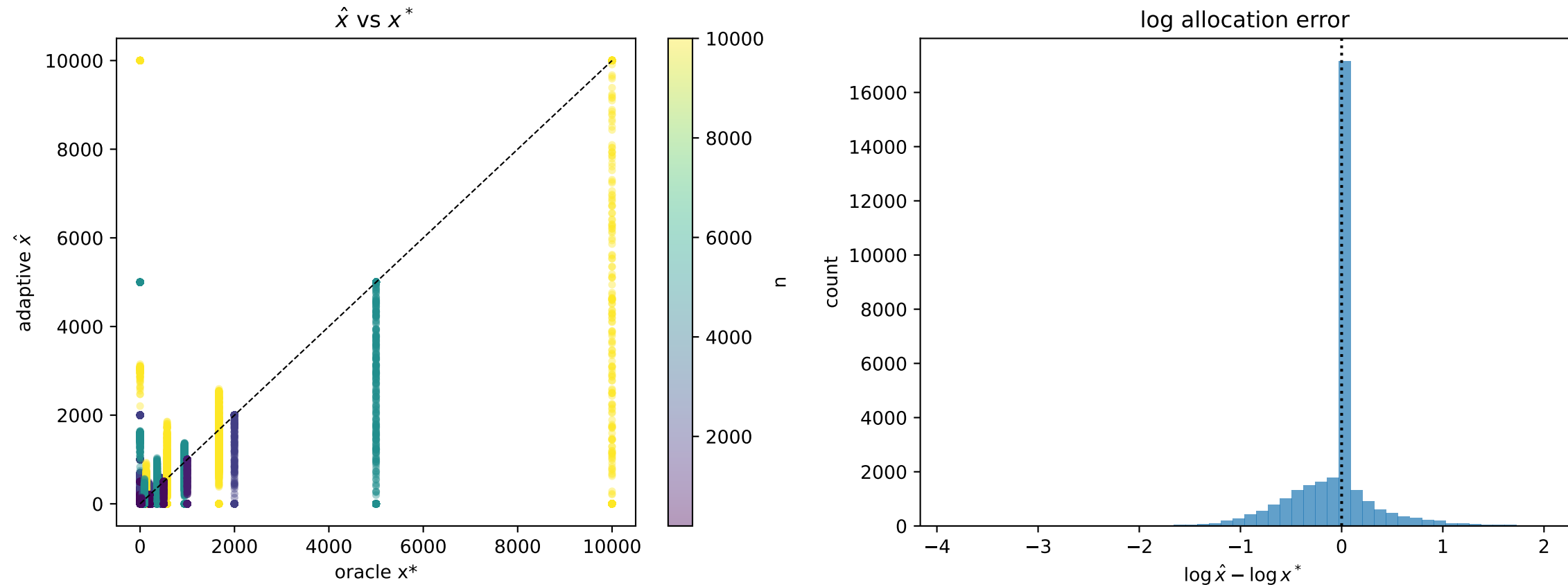
Figure A2: adaptive vs oracle allocation
