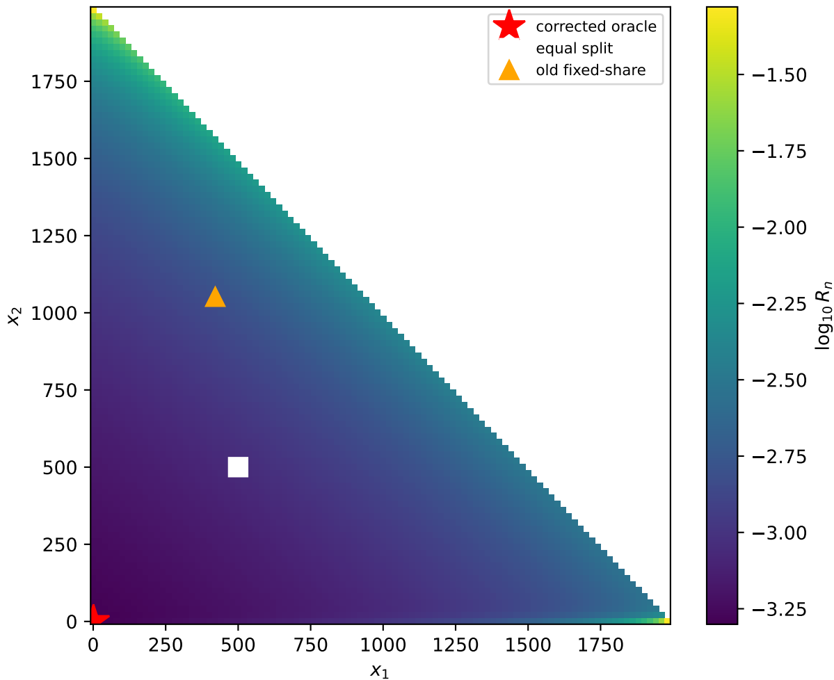
Figure M1: risk surface ( n=2000 , \beta_1=0.4 , \beta_2=1.0 )
