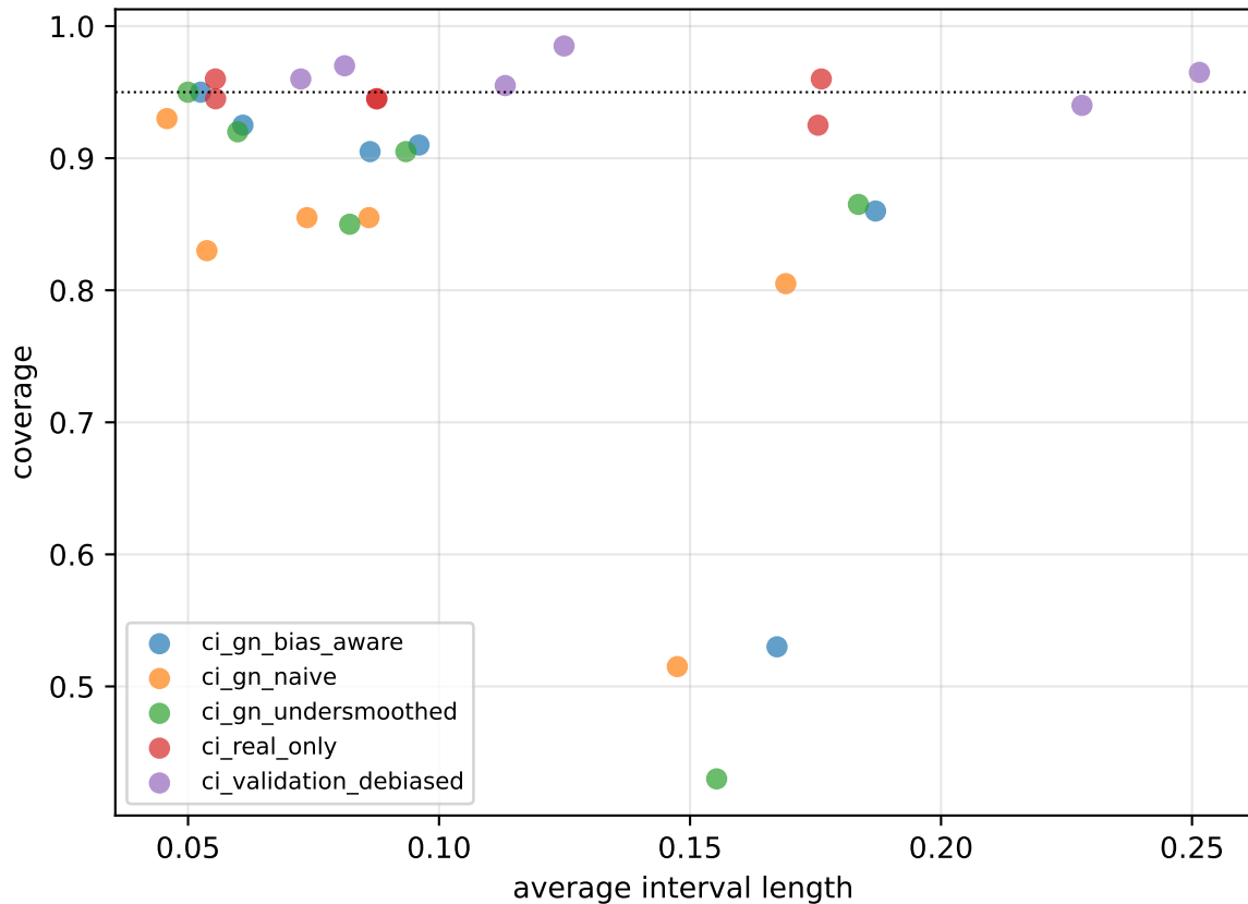
Figure C2: coverage vs interval length
