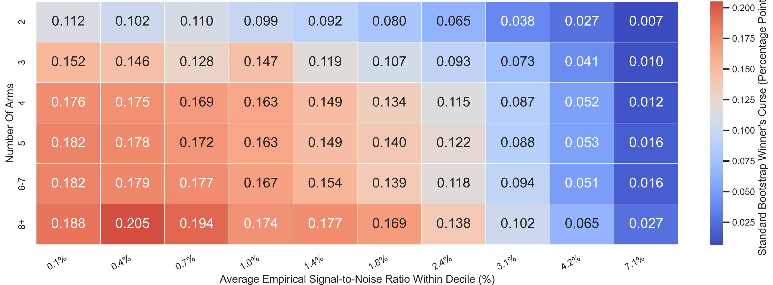
Winner's Curse By Arm Count And Average SNR
