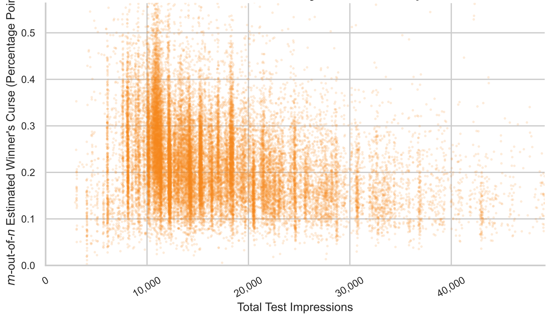
m -out-of- n Winner's Curse By Total Test Impressions
