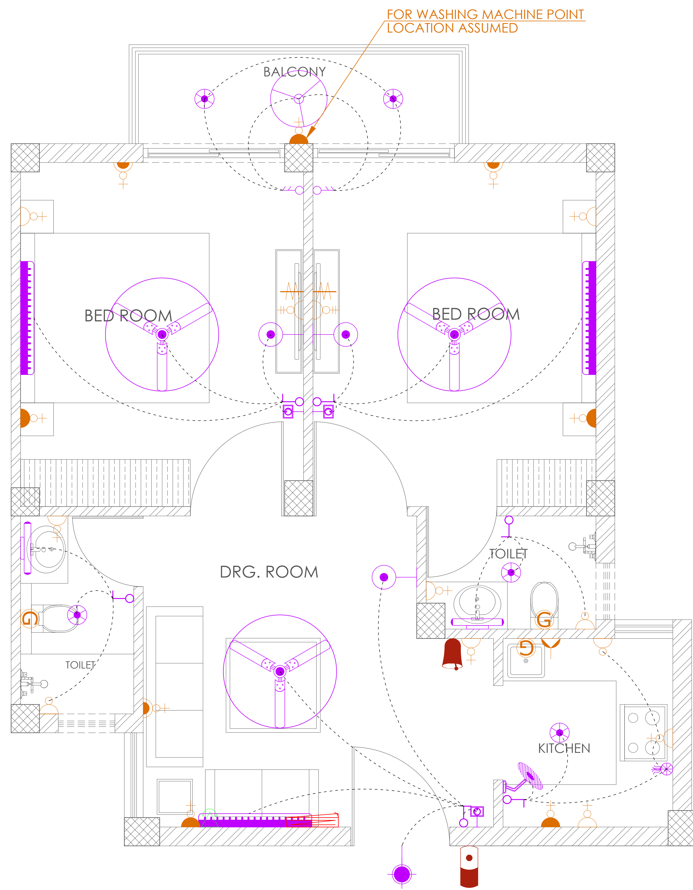
TYPICAL 2-BHK UNIT WORKING PLAN (FLOOR LAYOUT, UNIT WORKING PLAN)
