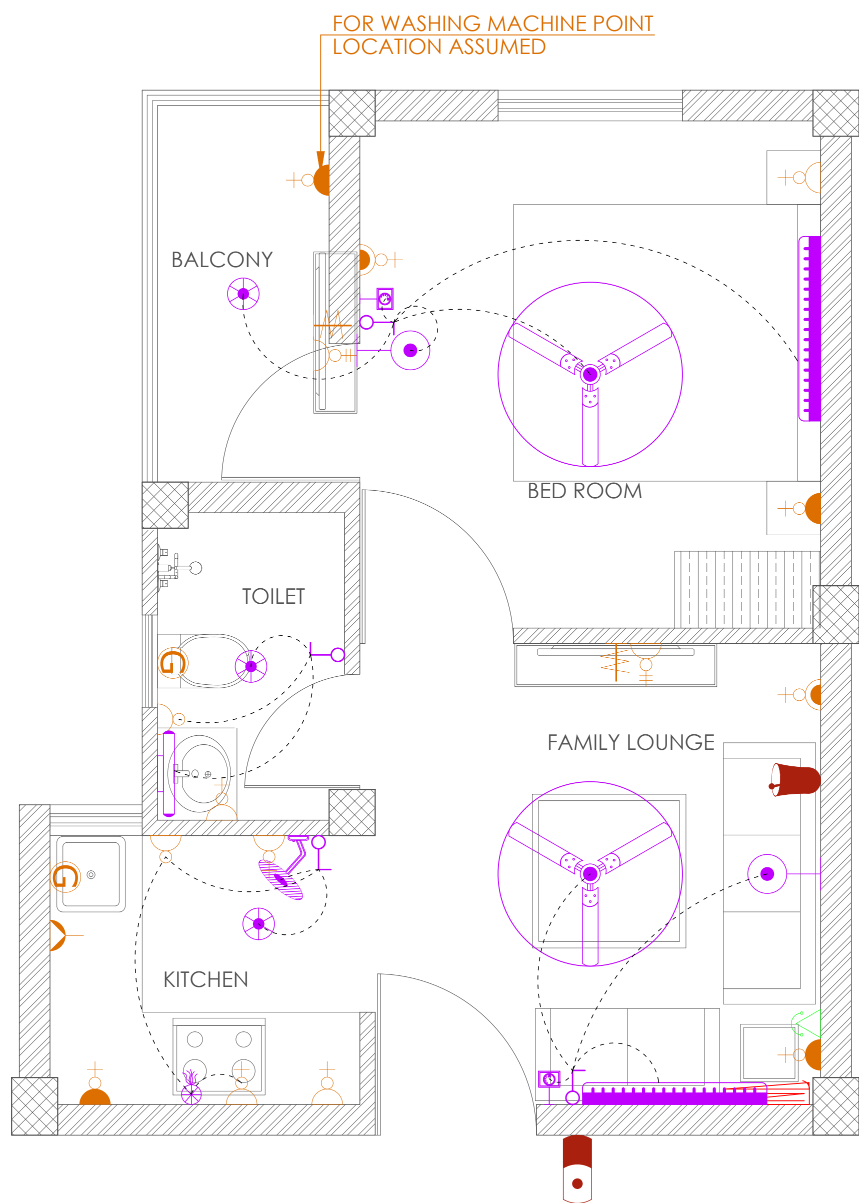
TYPICAL 1-BHK UNIT WORKING PLAN (FLOOR LAYOUT, UNIT WORKING PLAN)
