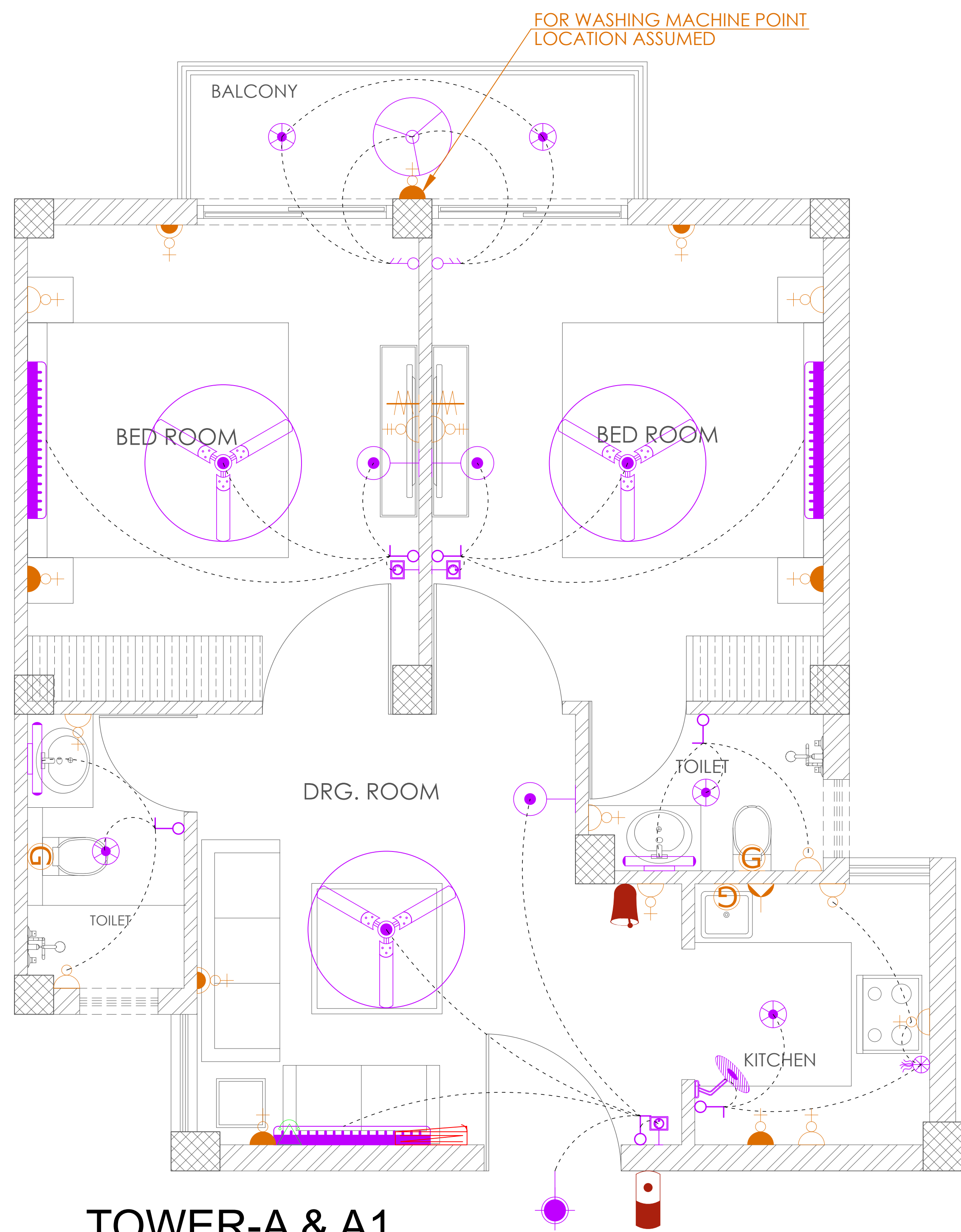
TOWER-A & A1 (FLOOR LAYOUT, UNIT WORKING PLAN)
