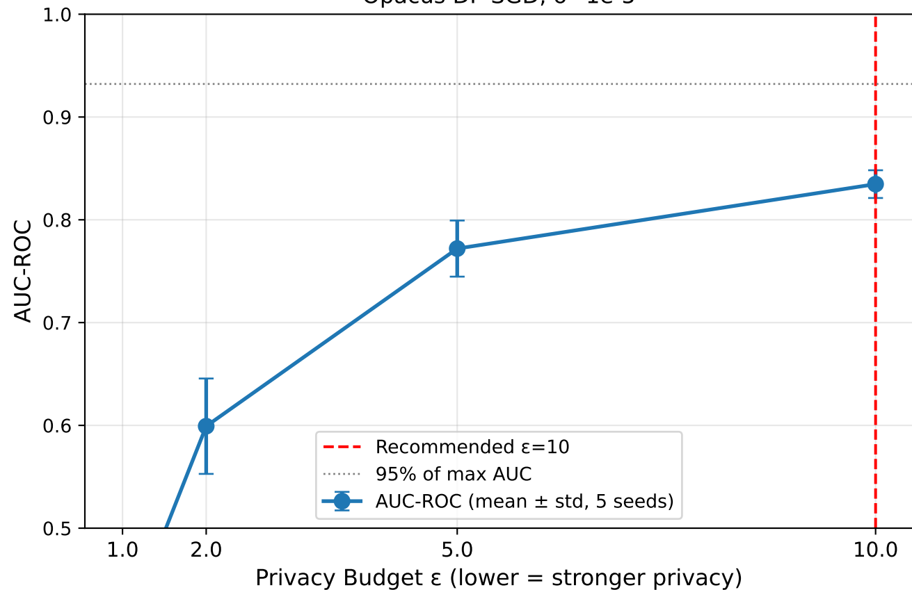
Privacy-Utility Tradeoff Curve (Figure 5) Opacus DP-SGD, \delta=1e-5
