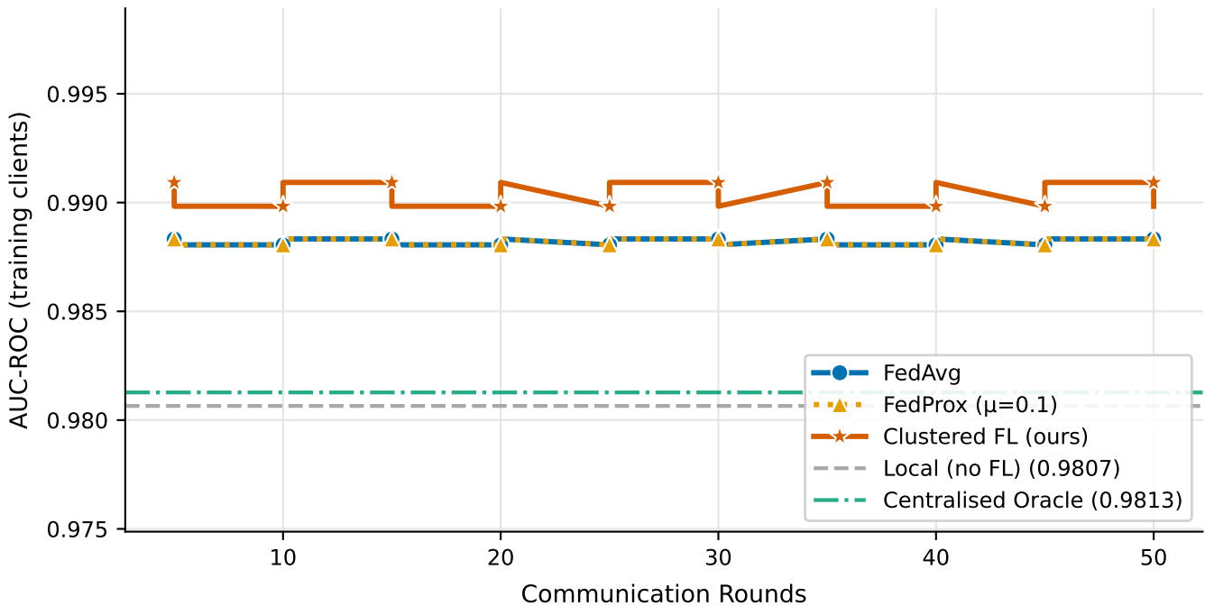
FL Convergence Curves — FedAcuity
