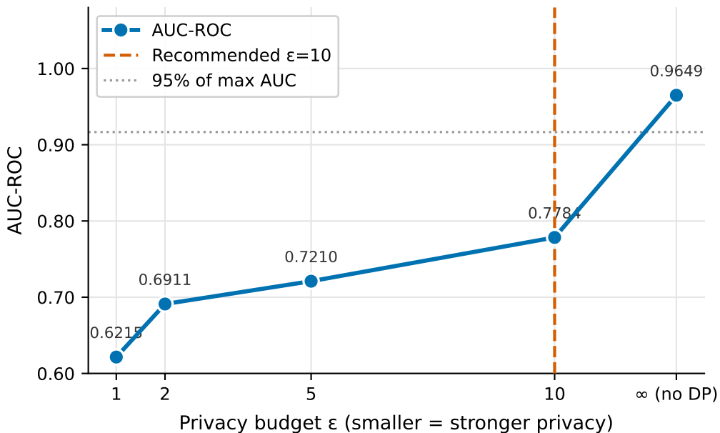
Privacy-Utility Tradeoff Curve (Figure 5) Opacus DP-SGD · StaffingNN · \delta=10^{-5}
