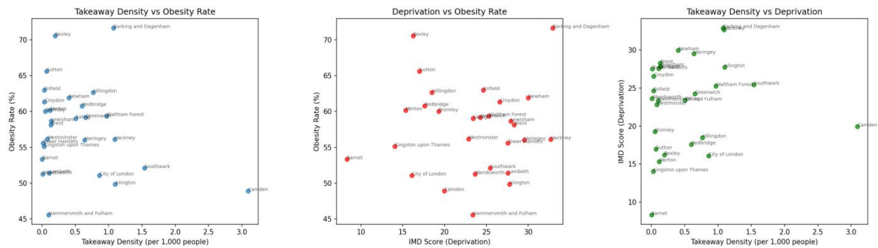
Figure 2: Scatterplots
