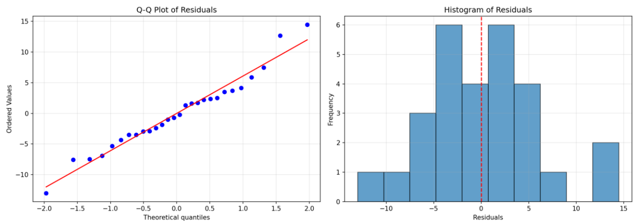
Figure 8: Normality Check.
