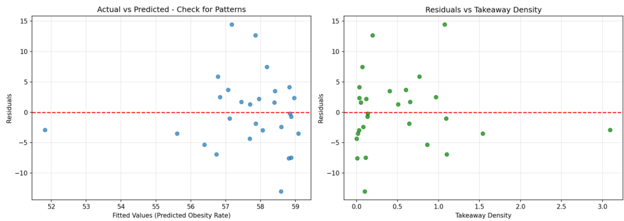
Figure 7: Linearity Check.
