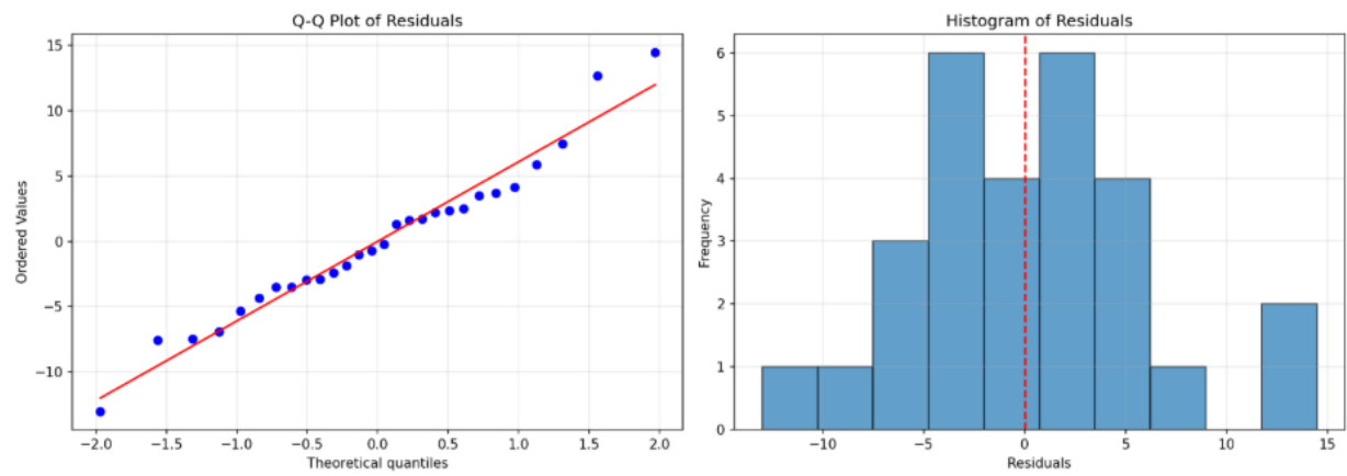
Figure 8: Normality Check.
