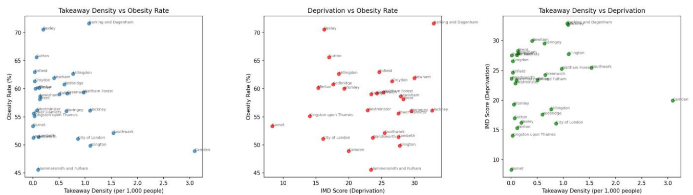
Figure 2: Scatterplots
