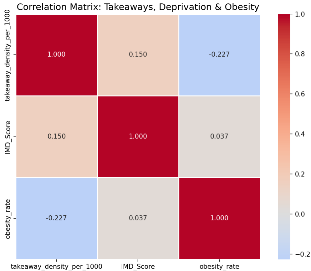
Figure 1: Correlation Matrix
