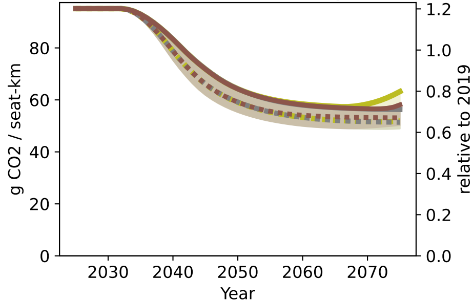
Carbon intensity
