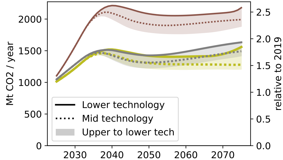
Carbon intensity
