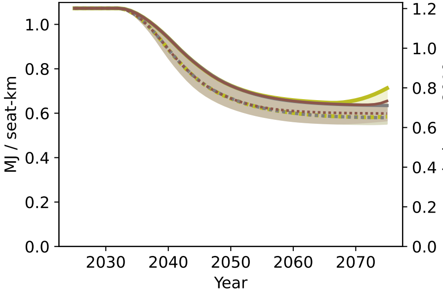
Energy intensity
