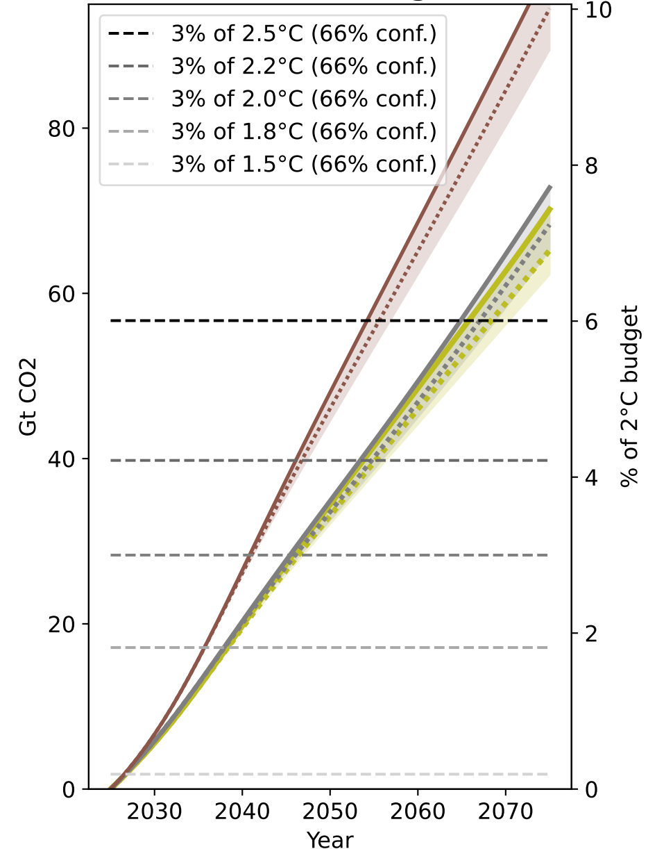
Carbon budget
