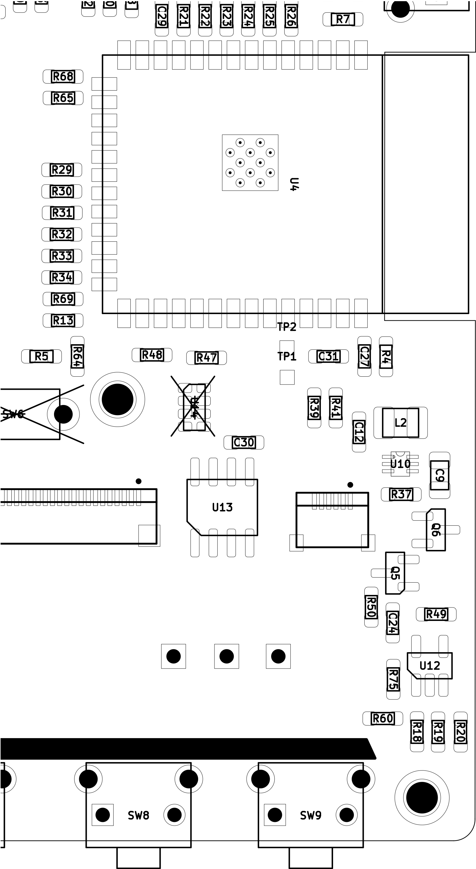
Detail 4 of 4: BOTTOM side, seen from below (mirrored), x6.5. Crossed-out parts are not fitted.
