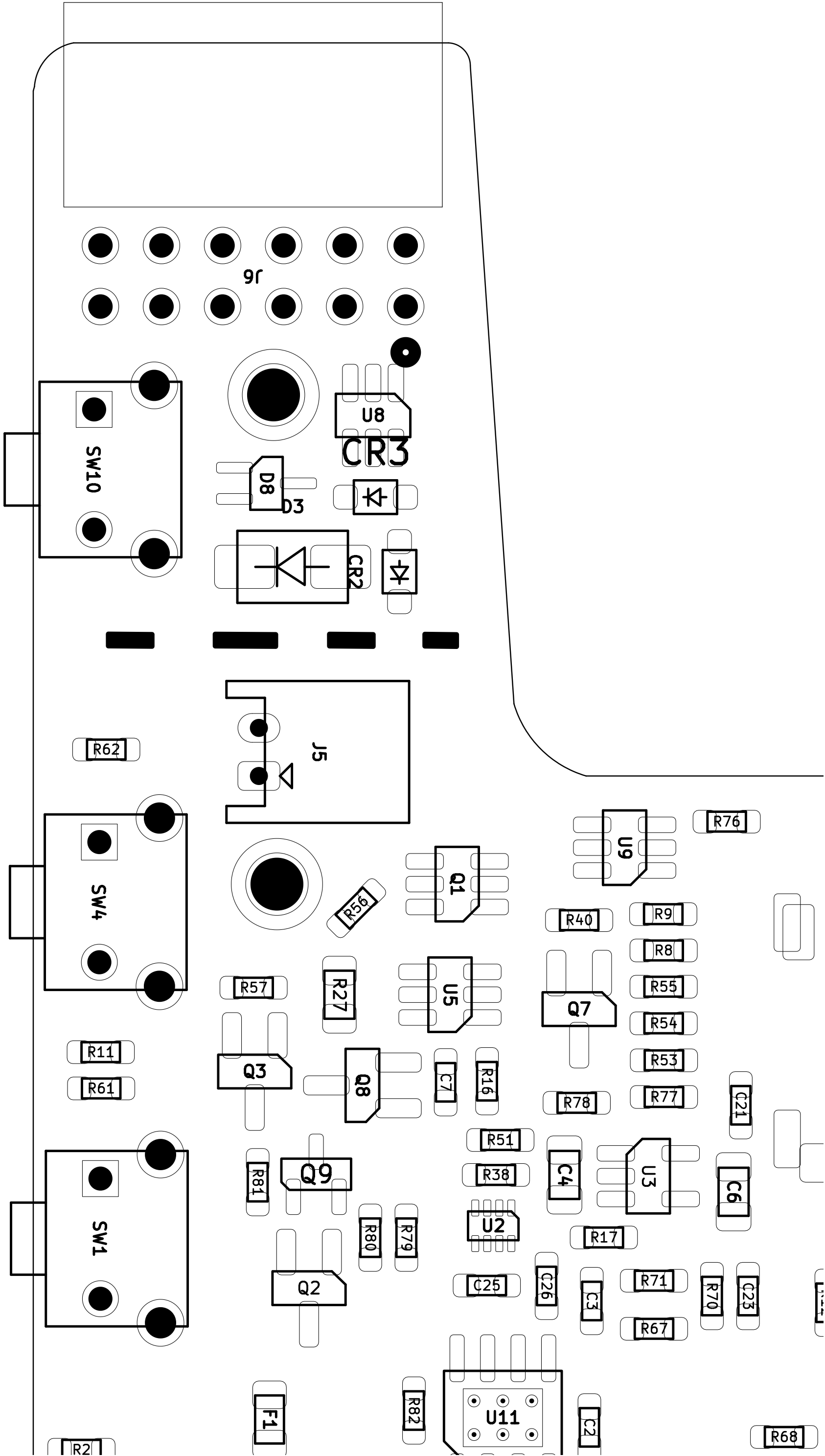
Detail 1 of 4: BOTTOM side, seen from below (mirrored), x6.5. Crossed-out parts are not fitted.
