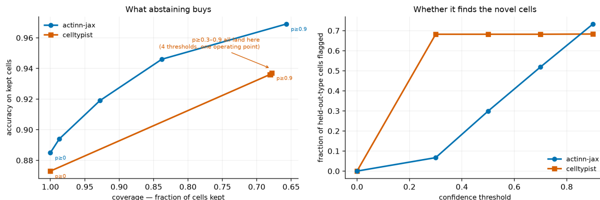
Figure 6. What abstention buys, and whether it finds the novel cells. Left: accuracy on kept cells against the fraction kept. Right: the share of held-out-type cells flagged as the threshold rises. actinn-jax traces a usable curve on both axes; CellTypist’s probabilities are saturated, so thresholds from 0.3 to 0.9 land on one operating point.
