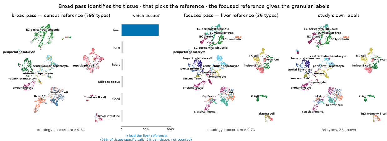
Figure 4. The workflow on a withheld HLiCA liver study (3,396 cells), same embedding throughout. Left : the shipped census reference spreads 137 of its 798 labels over the query (concordance
